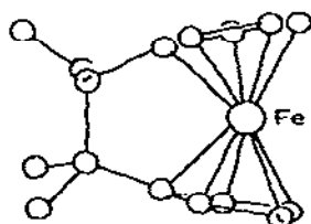
Fig. 6. The structure of 1,1'-tetramethylethyleneferrocene (45).
