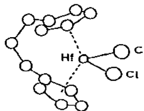
Fig. 8. The structure of (1,1'-trimethylenedicyclopentadienyl)hafnium chloride.
